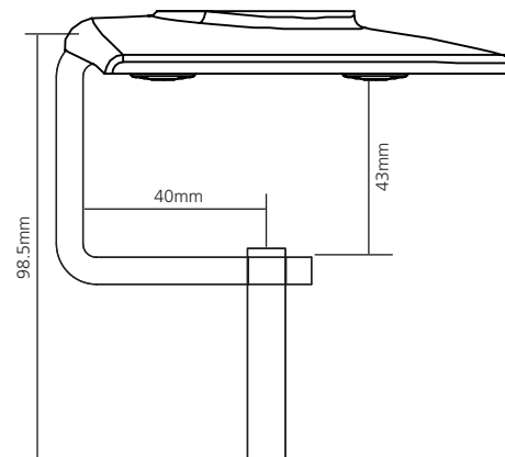
C clamp
