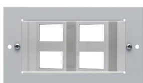
Angled plate pierced to accept 4 x LJ6C/RJ45 (Piercing 37.0 x 22.3)
