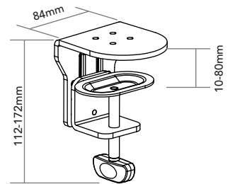
Double C-clamp used on 600mm pole
