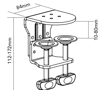
Double C-clamp used on 600mm pole
