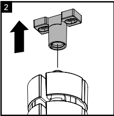
Carefully pull and separate the top fixing bracket from the top connecting block.
