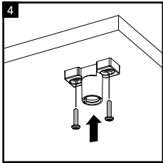
Use 2x suitable fixing screws to secure the top fixing bracket to the worksurface.
