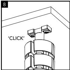
Push the block into the top fixing bracket until it clicks into place. Check it is secure.
