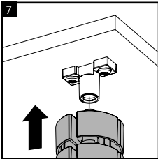
Offer up the top connecting block of the Rise to the top fixing bracket as shown.
