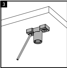
Use the top fixing bracket to mark the location of the fixing holes.
