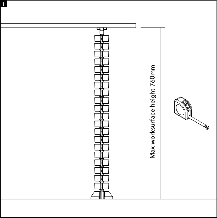
Measure the distance between the underside of the worksurface and the floor. Rise is to suit a max worksurface height of 760mm.
