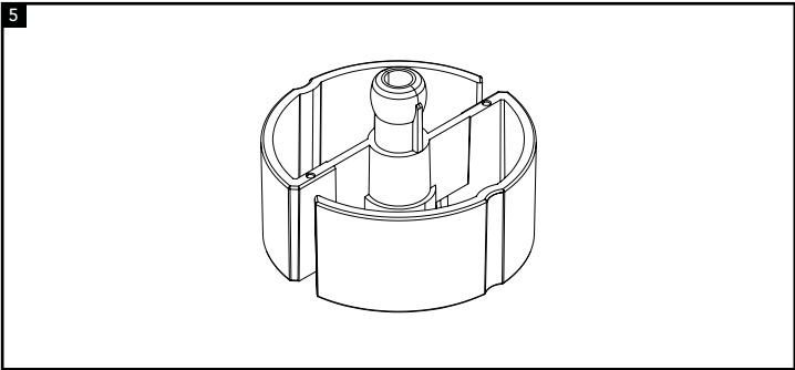
Each connecting block adds or removes 33mm to the height of the Rise.
