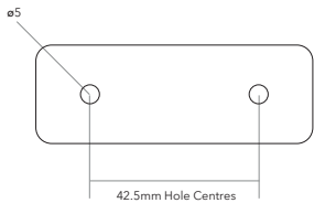
Desk fixing requires 2x fixing screws (supplied)
