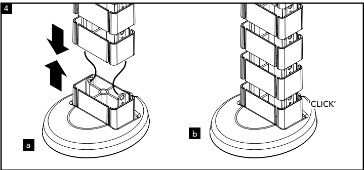
Orient the base to suit the cable entry as desired and offer up to the bottom connecting block (a). Push the bottom connecting block onto the base until it clicks into place (b).
