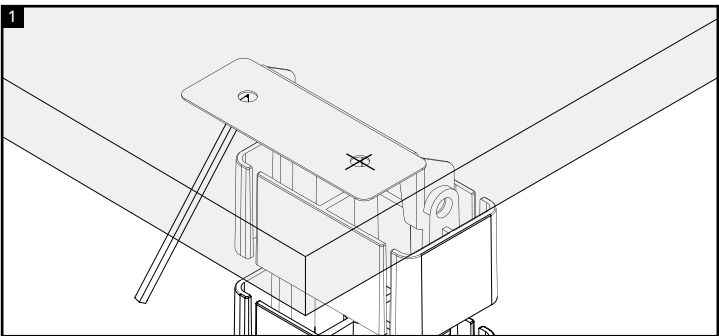
Use the mounting bracket to mark the fixing hole positions on the underside of the work surface.
