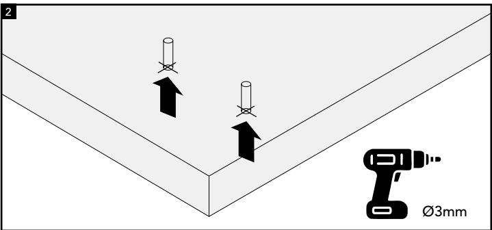
With a suitable tool, drill 2x 3mm pilot holes on the positions marked on the underside of the work surface.
