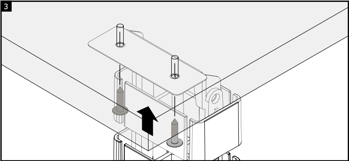
Use the 2x supplied fixing screws to fix the mounting bracket to the underside of the work surface as shown.
